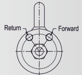
Mechanical Wedge Lock Arrangement with Anti Rotation
