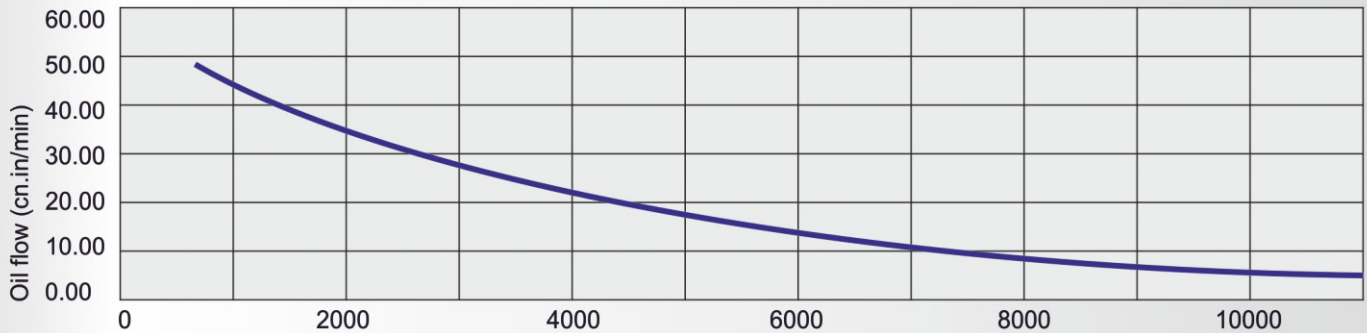
10000 PSI Air Hydraulic Pump Flow Rate
