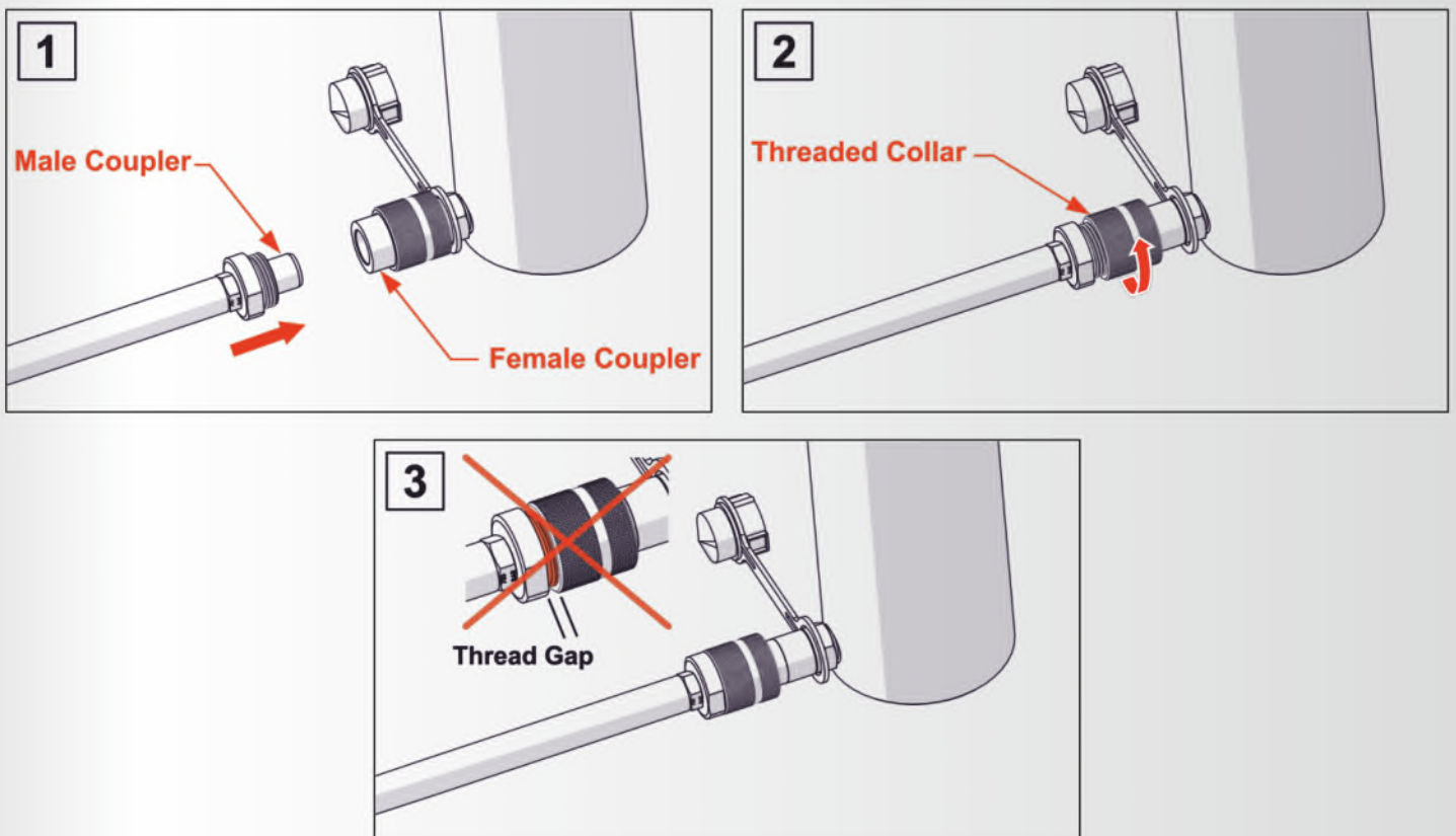
Figure 5.1: Hydraulic Connection
